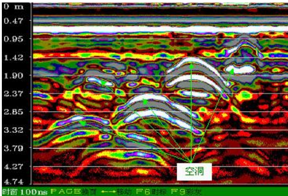
Survey image of Underground soil cave group
