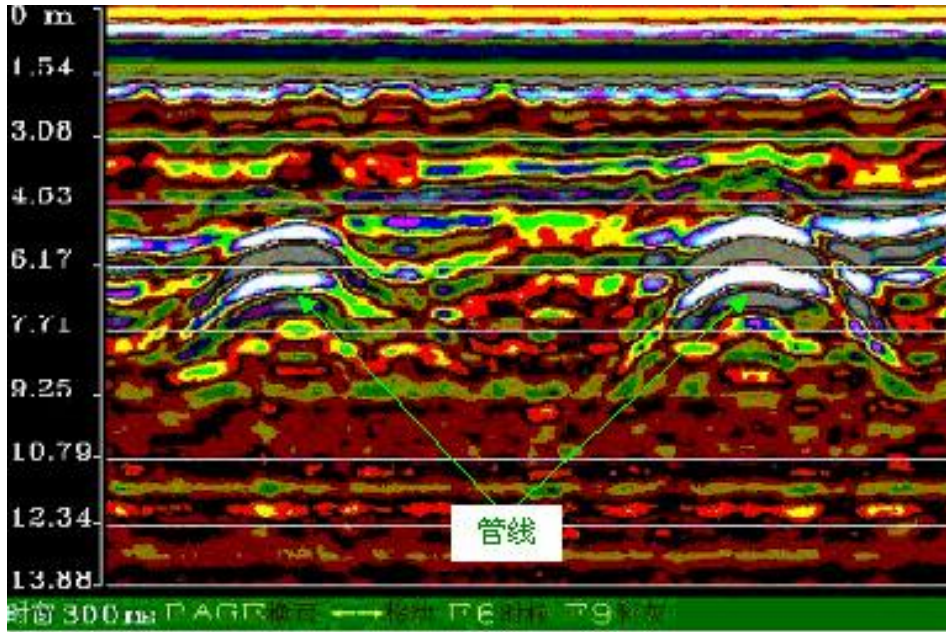
Underground pipeline survey image
