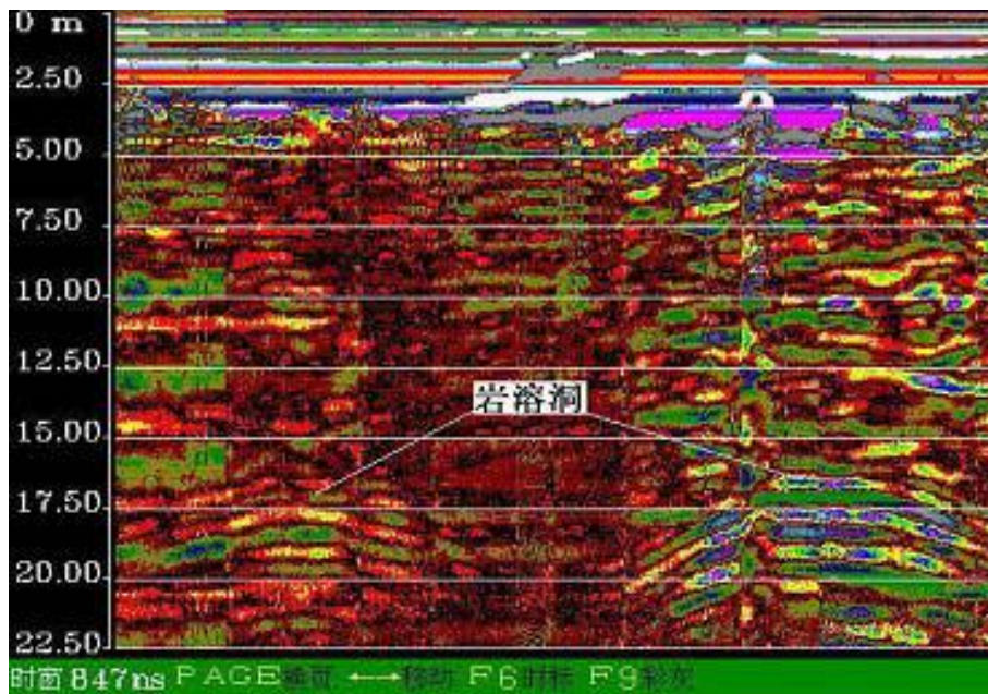
Karst cave survey image in limestone area
